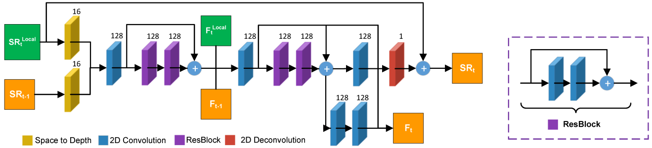
Figure 3: Architecture of the proposed NET_C . It produces the HR frame SR_t and feature F_t by exploiting the context information from previously predicted HR frames and features (i.e., SR_{t-1}, F_{t-1} ) and the outputs of NET_L (i.e., SR_t^{Local}, F_t^{Local} ).
